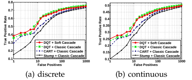
Fig. 13. Comparison of NPD face detectors based on different weak learners on the FDDB database [3] with (a) discrete and (b) continuous score metrics.
