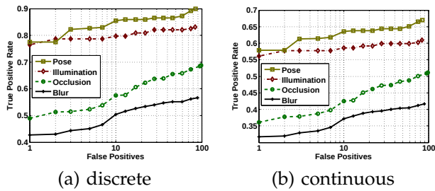
Fig. 15. ROC curves of the proposed NPD face detector on the four subsets extracted from the Fddb database [3] with (a) discrete and (b) continuous score metrics.
