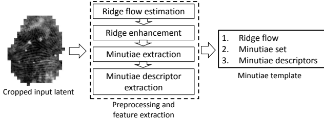
Fig. 6: Minutiae template generation. The same procedure is used for both minutiae template 1 and minutiae template 2.
