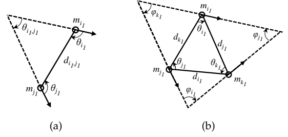
Fig. 9: Illustration of feature representation of (a) a minutiae pair (m_{i_1}, m_{j_1}) and (b) a minutiae triplet (m_{i_1}, m_{j_1}, m_{k_1}) , where the solid arrows denote minutiae orientations.
