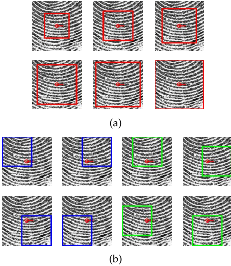
Fig. 8: Fourteen types of fingerprint patches, with different size and location, centered at a minutia (shown in red). Patches at (a) 6 different scales and (b) in 8 different locations around minutia: top left, top right, bottom right and bottom left, top, right, left and bottom. The fingerprint patches shown here are of size 160 \times 160 pixels. The window sizes (scale) in (a) are 80 \times 80 , 96 \times 96 , 112 \times 112 , 128 \times 128 , 144 \times 144 , and 160 \times 160 pixels. The windows in (b) are all of size 96 \times 96 pixels.
