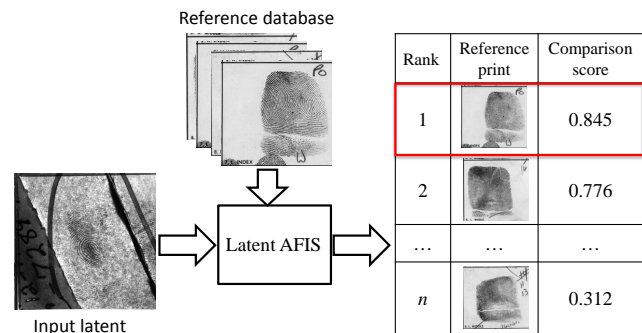
Fig. 1: Automated latent recognition framework. A latent image is input to a latent AFIS, and the top n candidates with their comparison scores are presented to a latent expert. The number of candidates, n , examined is typically less than 20. The true mate in this example is outlined in red.
