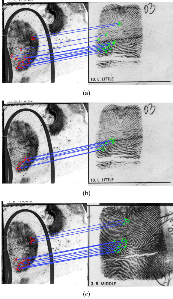
Fig. 10: Comparison of minutiae correspondences. (a) 14 minutiae pairs found in correspondence between the latent and a non-mate [30], (b) 7 minutiae pairs found in correspondence for the same comparison as in (a) by the proposed method and (c) 13 minutiae pairs found in correspondences between the latent and its true mate by the proposed method. Note that we use manually marked minutiae and MCC descriptor [39] for a fair comparison with [30].
