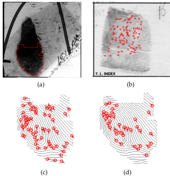
Fig. 14: A latent whose true mate was retrieved at rank-1 by minutiae template 1 but not by minutiae template 2 (rank-2,457). (a) Input latent with its ROI (G044 from NIST SD27), (b) mated reference print of (a) with overlaid minutiae, (c) minutiae set 1 of (a) overlaid on latent skeleton, and (d) minutiae set 2 of (a) overlaid on latent skeleton.
