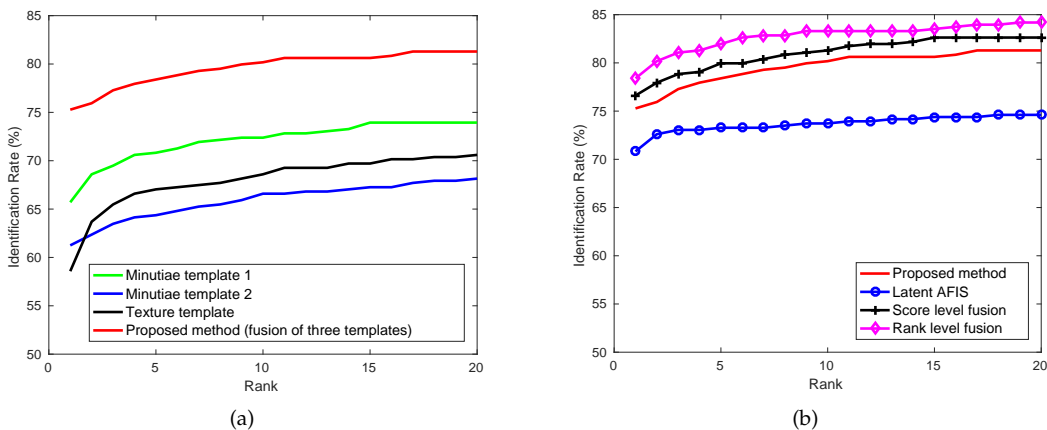
Fig. 13: Cumulative Match Characteristic (CMC) curves for WVU DB of (a) individual templates (minutiae template 1, minutiae template 2 and texture template) and their fusion, and (b) comparison of the proposed method with a COTS latent AFIS and score-level and rank-level fusion of the proposed method and COTS latent AFIS.
