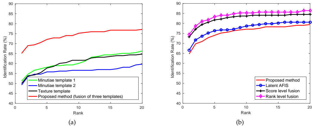
Fig. 12: Cumulative Match Characteristic (CMC) curves for NIST SD27 of (a) individual templates (minutiae template 1, minutiae template 2 and texture template) and their fusion, and (b) comparison of the proposed method with a COTS latent AFIS and score-level and rank-level fusion of the proposed method and COTS latent AFIS.
