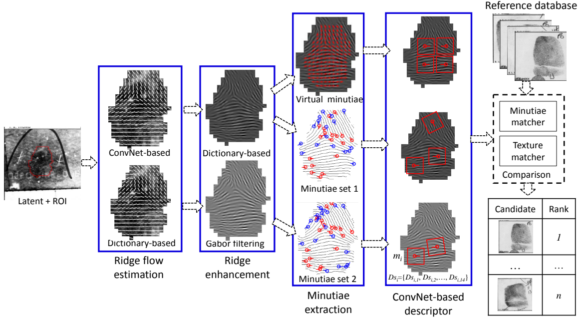
Fig. 5: Flowchart of the proposed latent recognition approach. The common minutiae in two true minutiae sets are shown in red.
