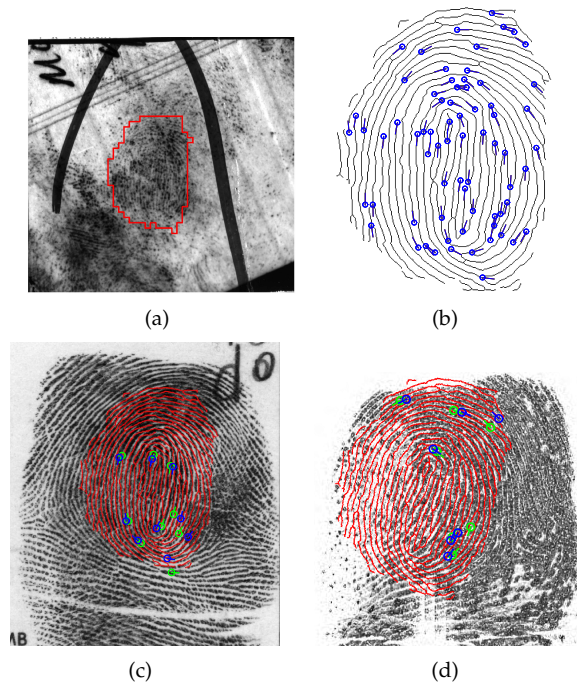
Fig. 2: Illustration of latent to reference (rolled) comparison. (a) Input latent with ROI outlined in red, (b) automatically extracted minutiae in (a) shown on the latent skeleton, (c) alignment and minutiae correspondences between the latent and its true mate (rank-1 retrieval) and (d) alignment and minutiae correspondences between the latent and the rank-2 retrieved rolled print. Blue circles denote latent minutiae and green circles denote rolled minutiae.
