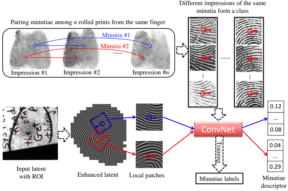
Fig. 7: Minutiae descriptor extraction via ConvNet. The dotted arrows show the offline training process, while solid arrows show the online process for minutiae descriptor extraction. A total of 800K fingerprint patches from 50K minutiae, extracted from the MSP longitudinal fingerprint database [33], were used for training the ConvNet. The patch size shown here is 80 \times 80 pixels.
