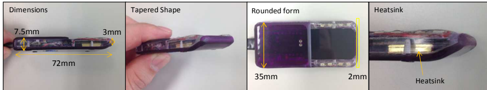
Fig. 41: ZAK-108 packaging design
