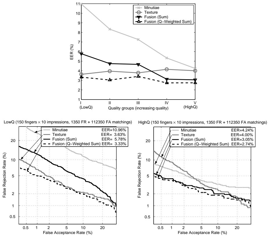
Fig. 4. Verification performance of the individual matchers (minutiae- and texture-based), their combination through the sum fusion fusion rule, and the proposed quality-based weighted sum for increasing image quality.
